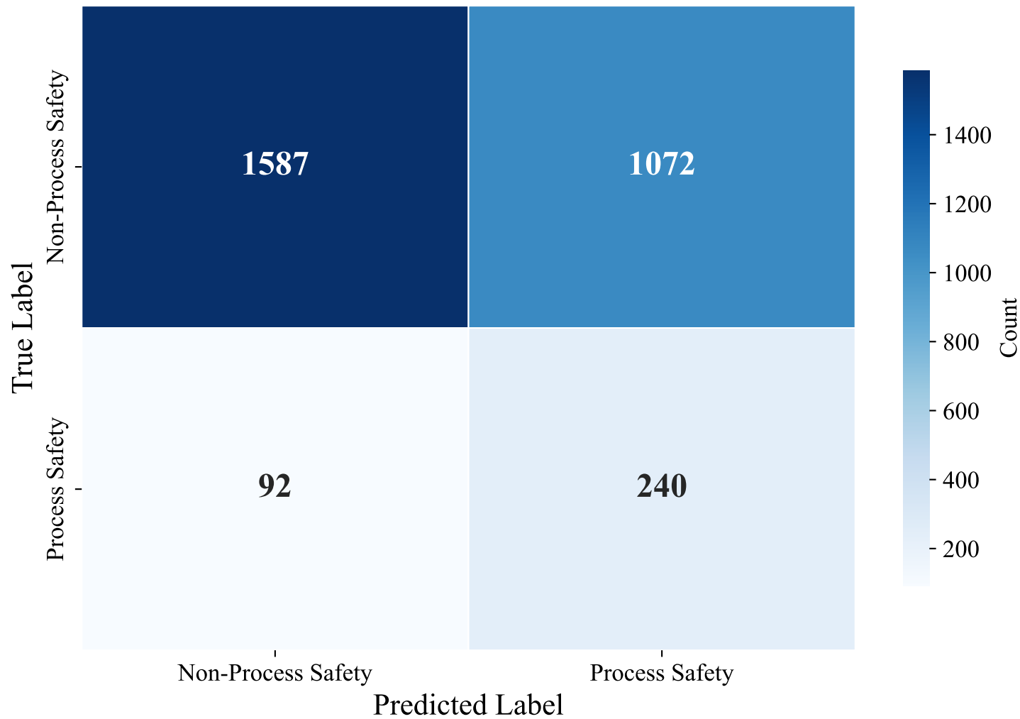
Confusion Matrix — GERMAN_MANUAL (paraphrase-multilingual-MiniLM-L12-v2, Random_Forest)
