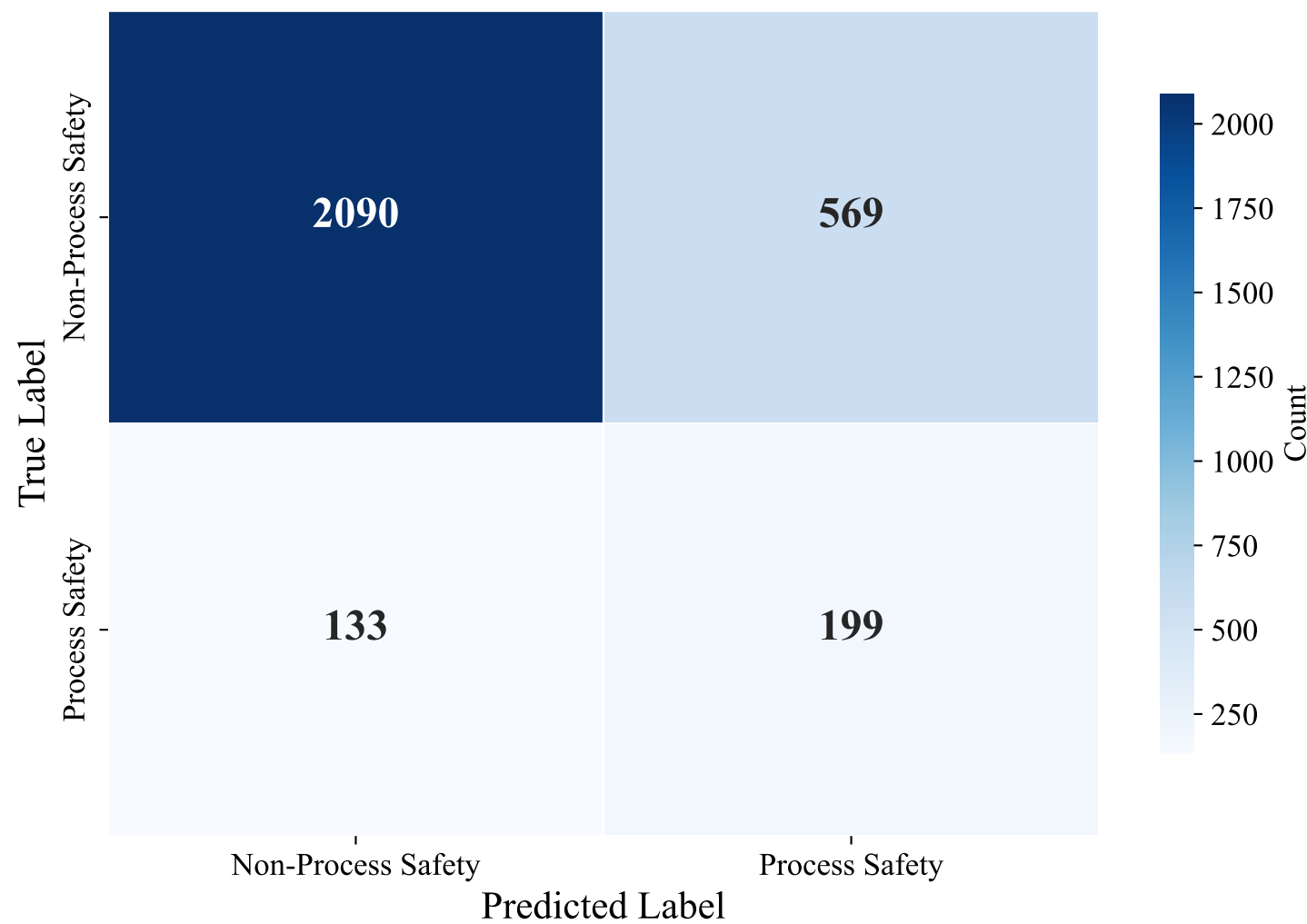
Confusion Matrix — GERMAN_MANUAL (paraphrase-multilingual-MiniLM-L12-v2, Voting_Ensemble)
