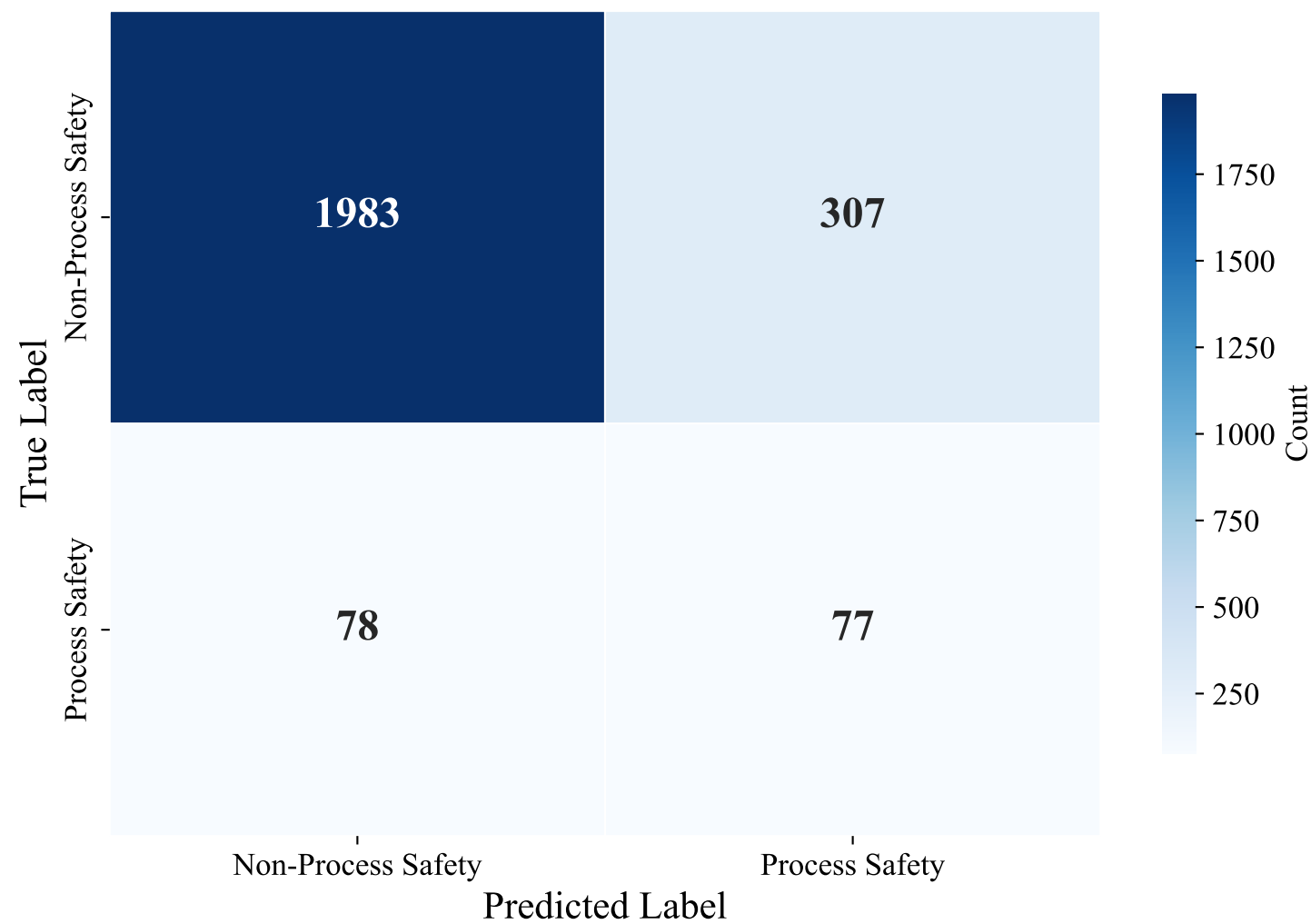
Confusion Matrix — SWEDISH_MANUAL (paraphrase-multilingual-MiniLM-L12-v2, Voting_Ensemble)
