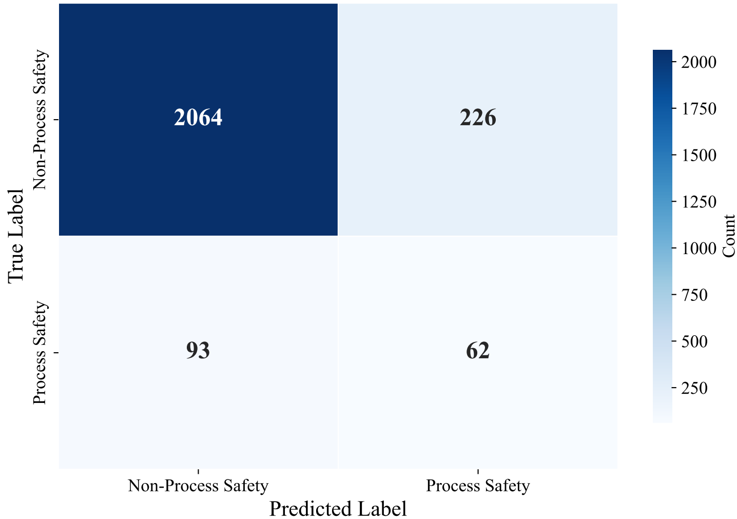
Confusion Matrix — SWEDISH_MANUAL (paraphrase-multilingual-mpnet-base-v2, XGBoost_Optimized)
