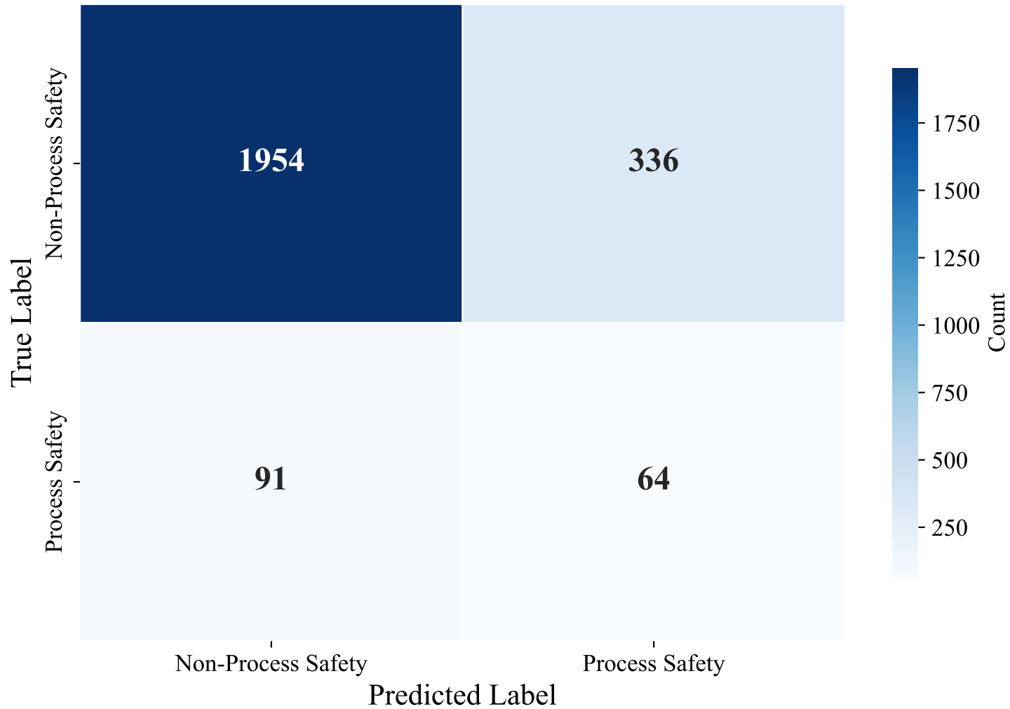
Confusion Matrix — SWEDISH_MANUAL (snowflake-arctic-embed-l-v2.0, SVM)
