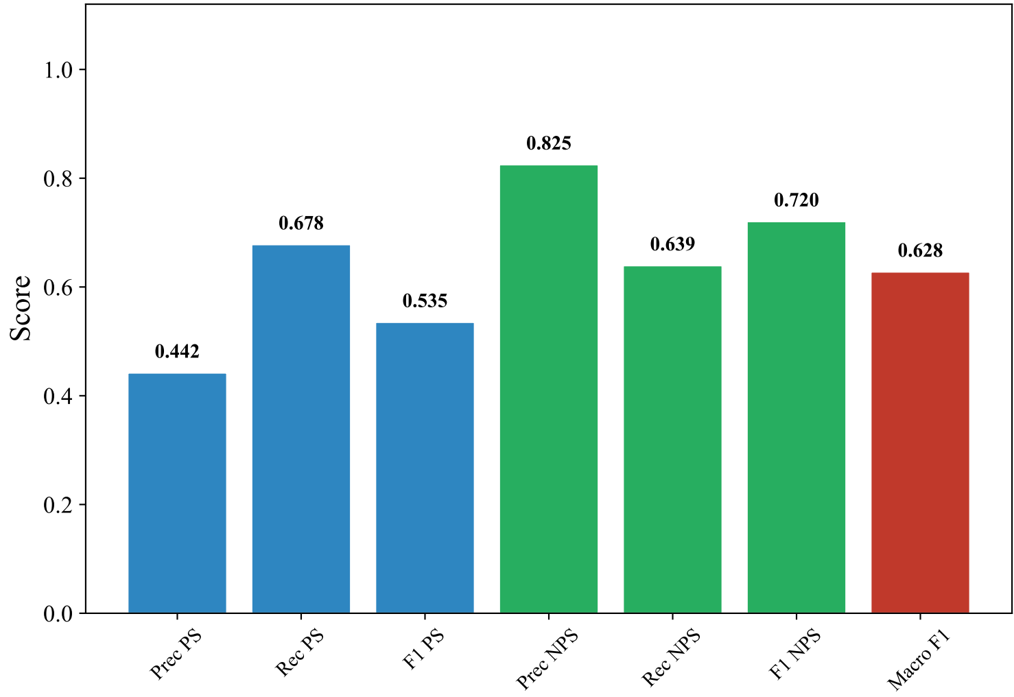
Classification Metrics — DUTCH_MANUAL (paraphrase-multilingual-MiniLM-L12-v2, SVM)
