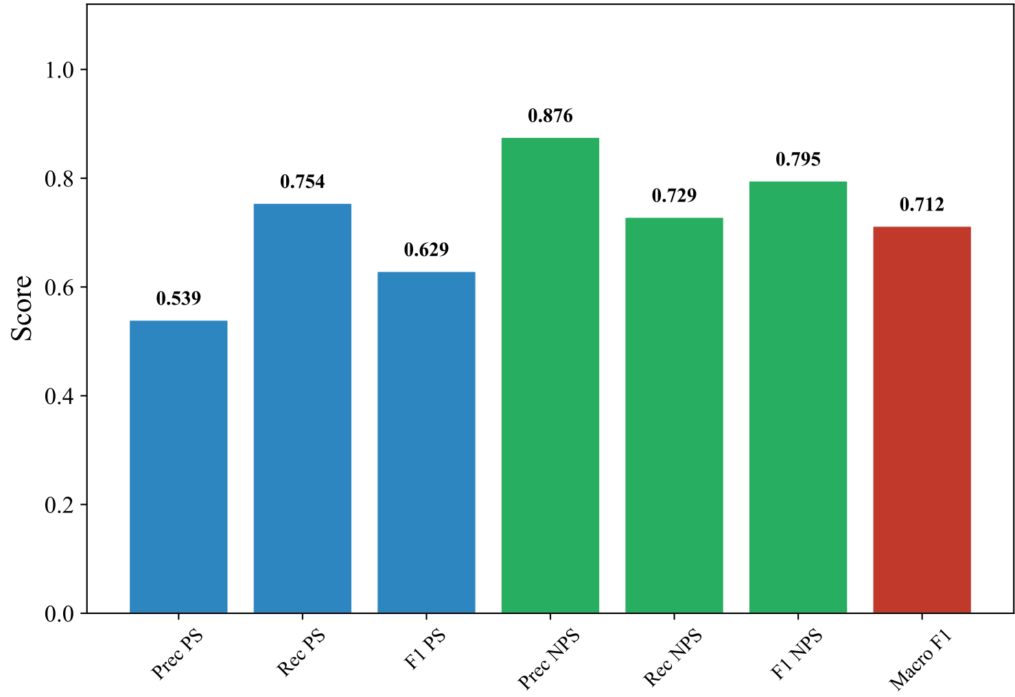
Classification Metrics — DUTCH_MANUAL (paraphrase-multilingual-mpnet-base-v2, LightGBM)
