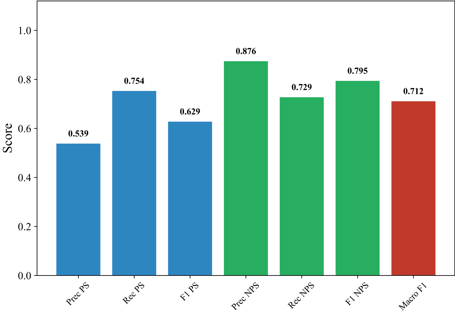
Classification Metrics — DUTCH_MANUAL (paraphrase-multilingual-mpnet-base-v2, LightGBM_Optimized)
