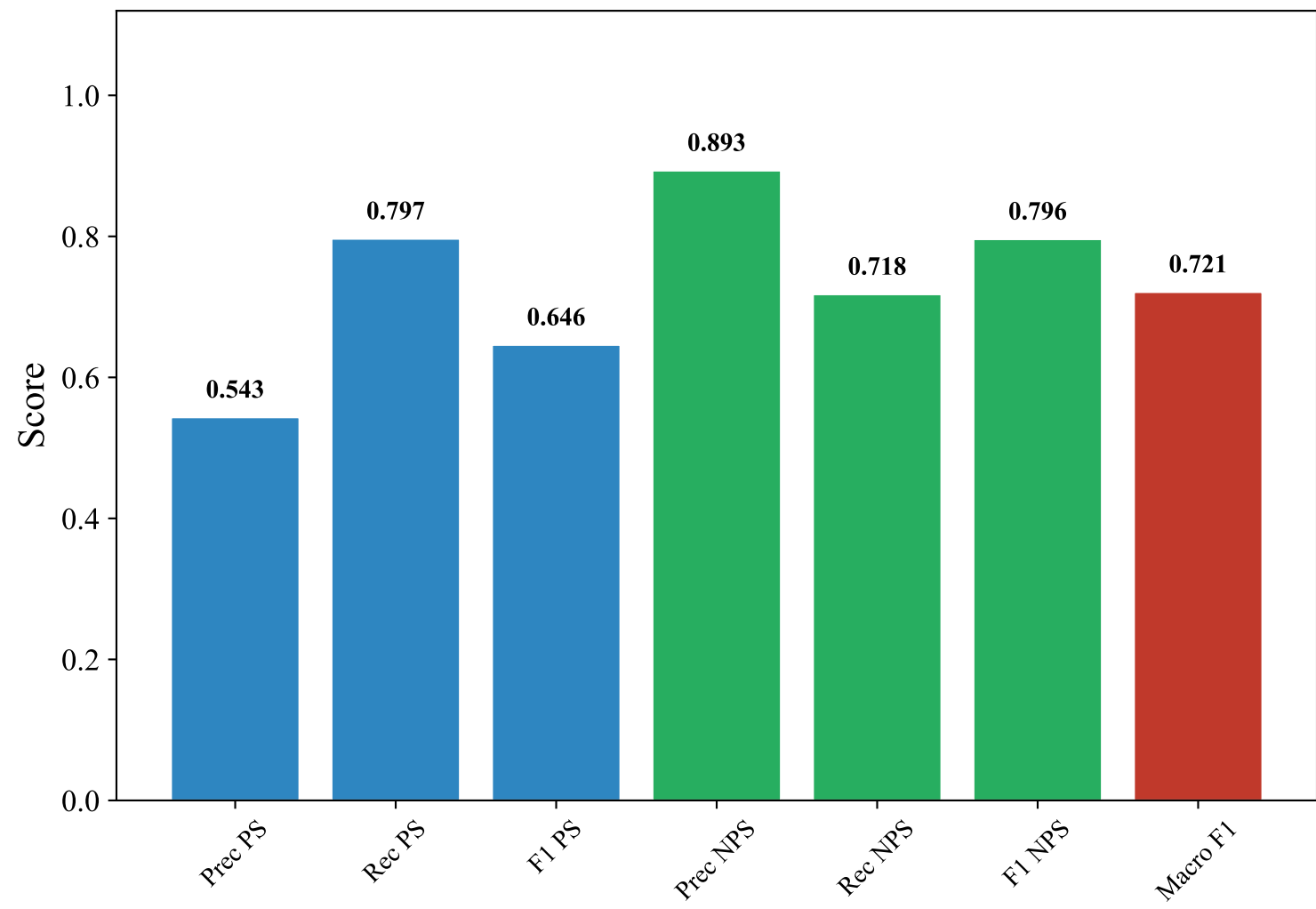
Classification Metrics — DUTCH_MANUAL (snowflake-arctic-embed-l-v2.0, Voting_Ensemble)
