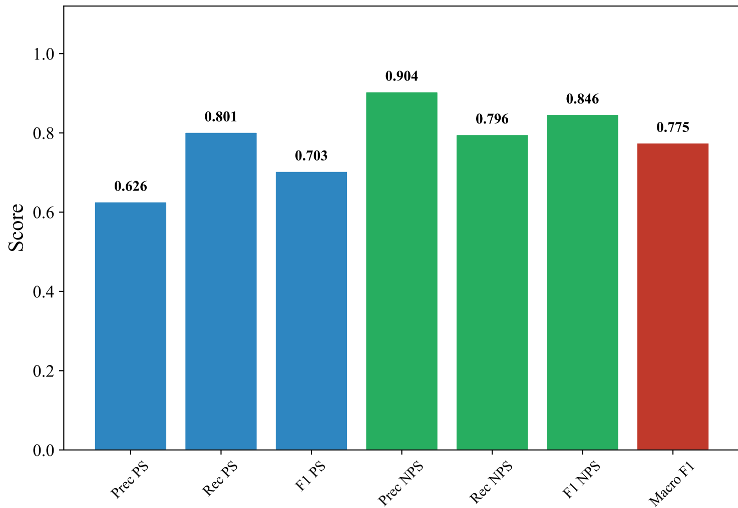
Classification Metrics — ENGLISH_MANUAL (snowflake-arctic-embed-l-v2.0, LightGBM_Optimized)
