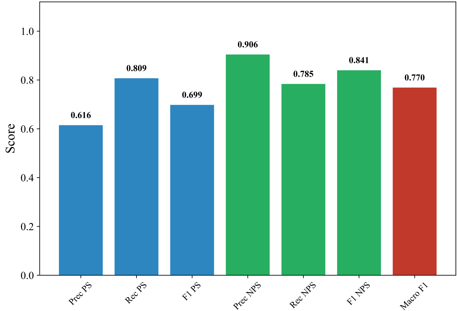
Classification Metrics — ENGLISH_MANUAL (snowflake-arctic-embed-l-v2.0, Voting_Ensemble)
