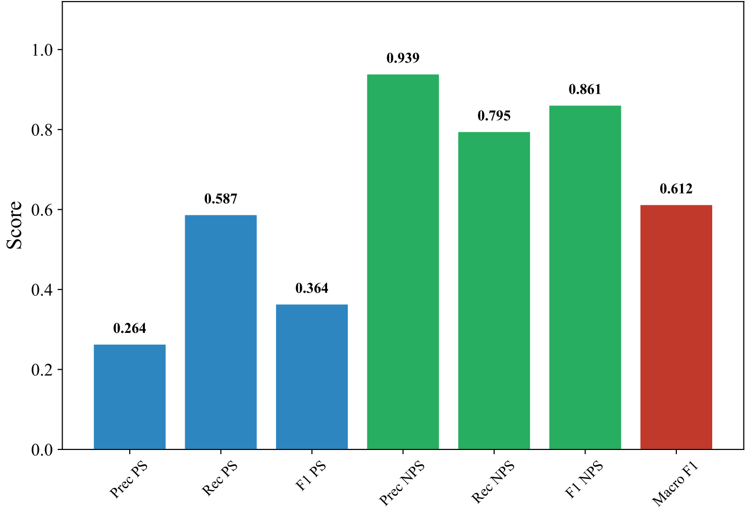
Classification Metrics — GERMAN_MANUAL (paraphrase-multilingual-MiniLM-L12-v2, LightGBM_Optimized)
