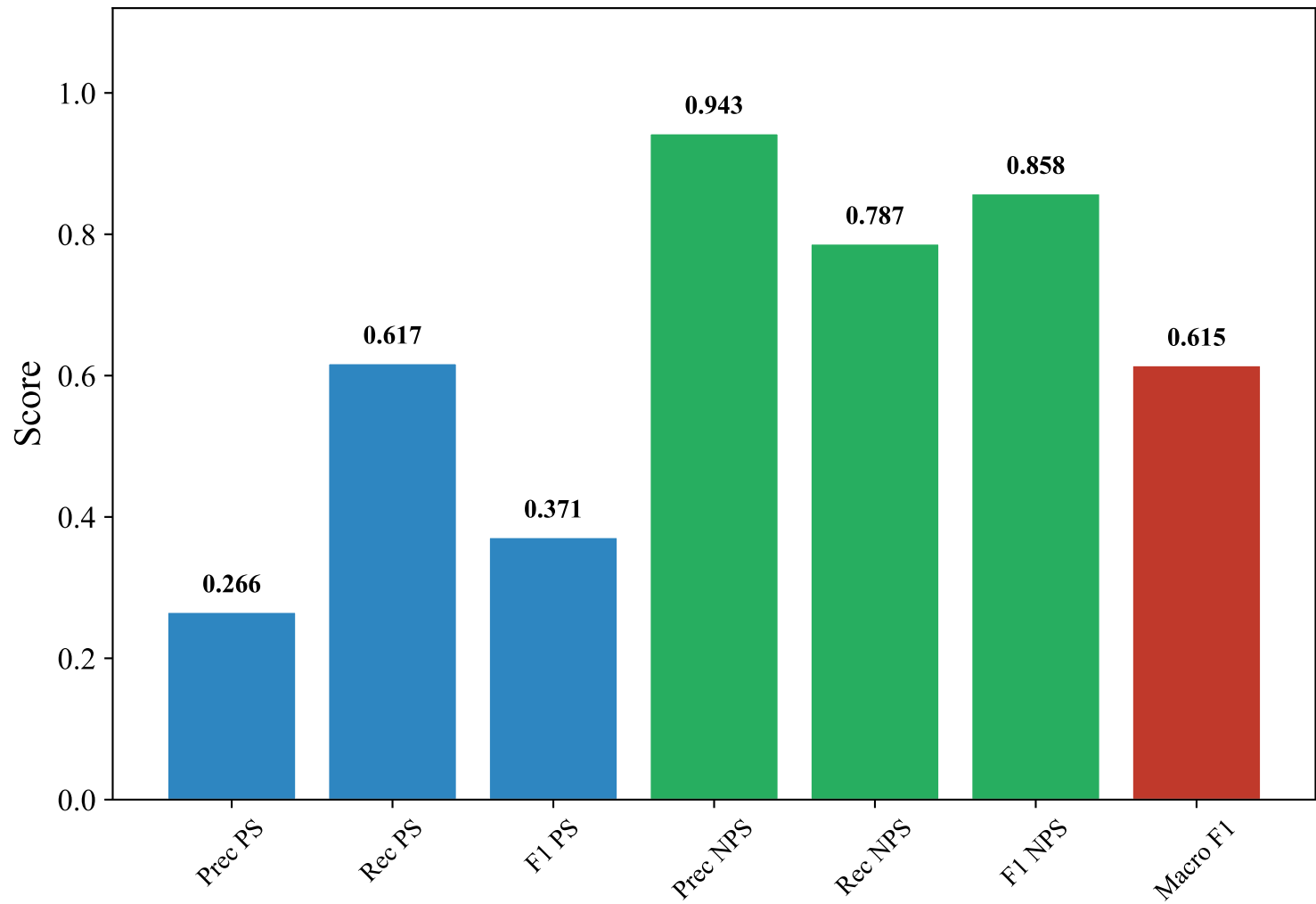
Classification Metrics — GERMAN_MANUAL (paraphrase-multilingual-MiniLM-L12-v2, SVM)
