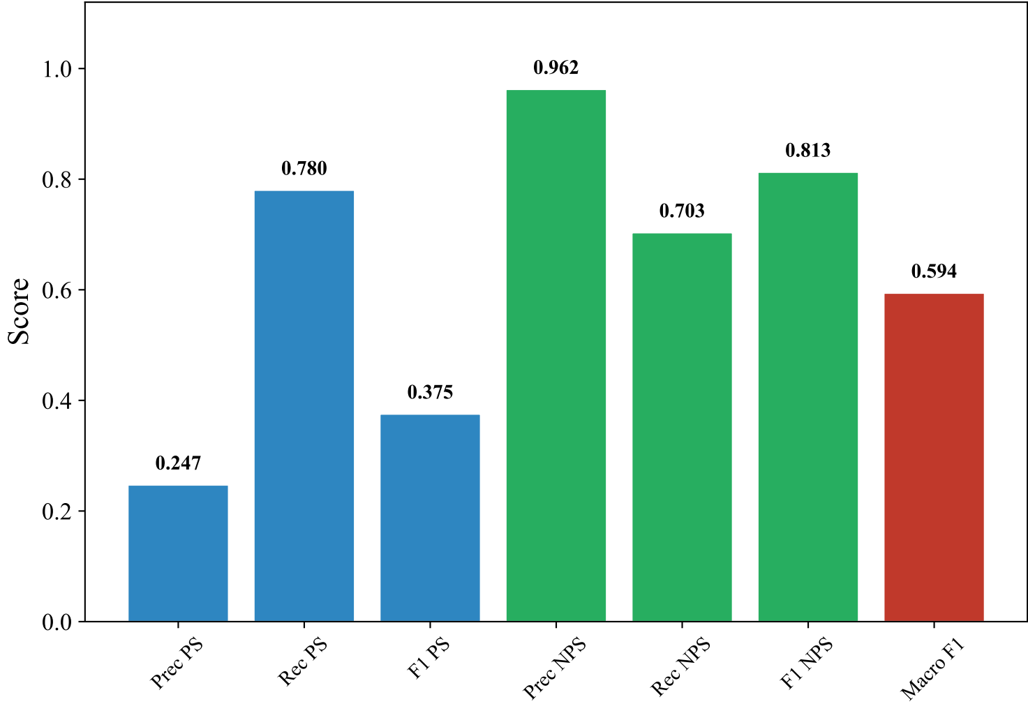
Classification Metrics — GERMAN_MANUAL (snowflake-arctic-embed-l-v2.0, Random_Forest)
