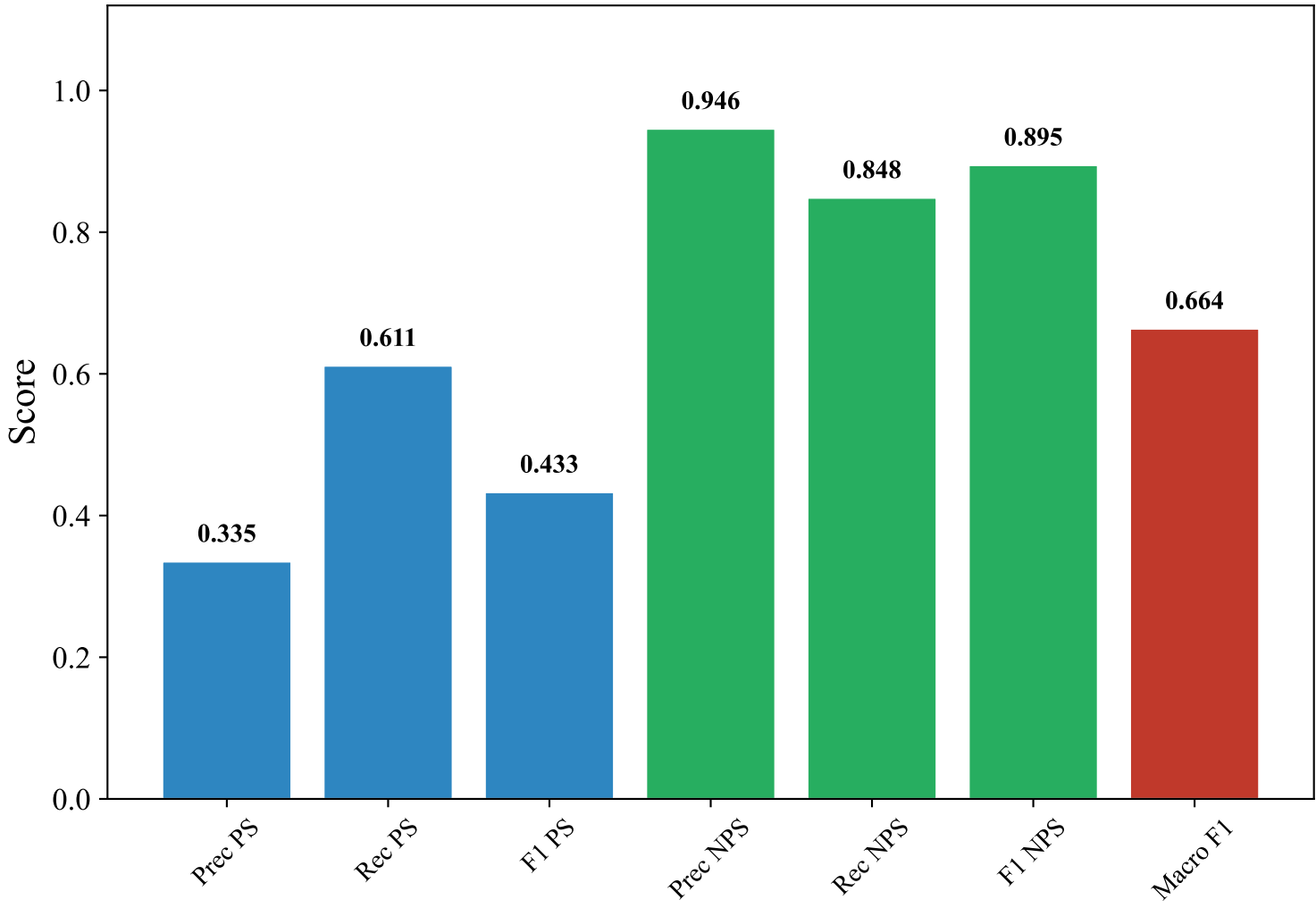
Classification Metrics — GERMAN_MANUAL (snowflake-arctic-embed-l-v2.0, SVM)
