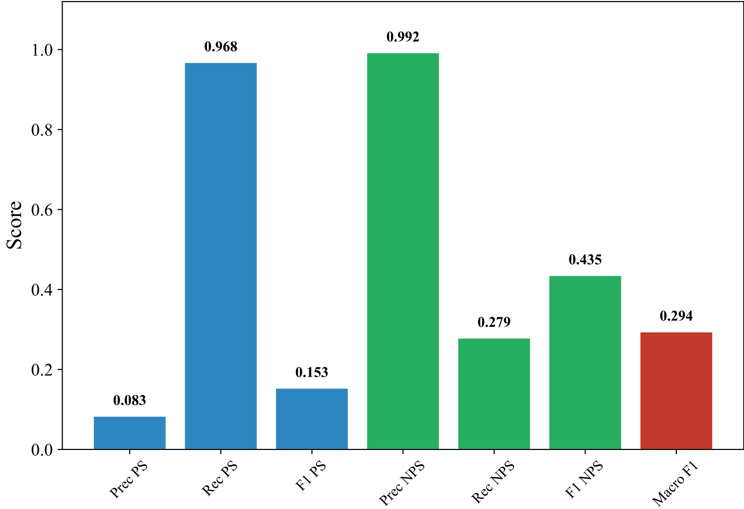
Classification Metrics — SWEDISH_MANUAL (paraphrase-multilingual-mpnet-base-v2, Random_Forest_Optimized)
