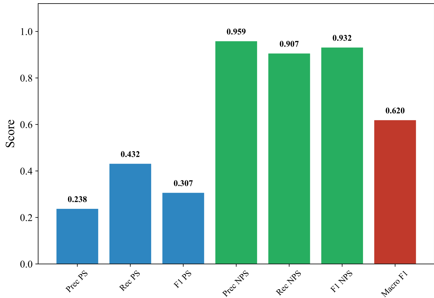
Classification Metrics — SWEDISH_MANUAL (snowflake-arctic-embed-l-v2.0, LightGBM_Optimized)
