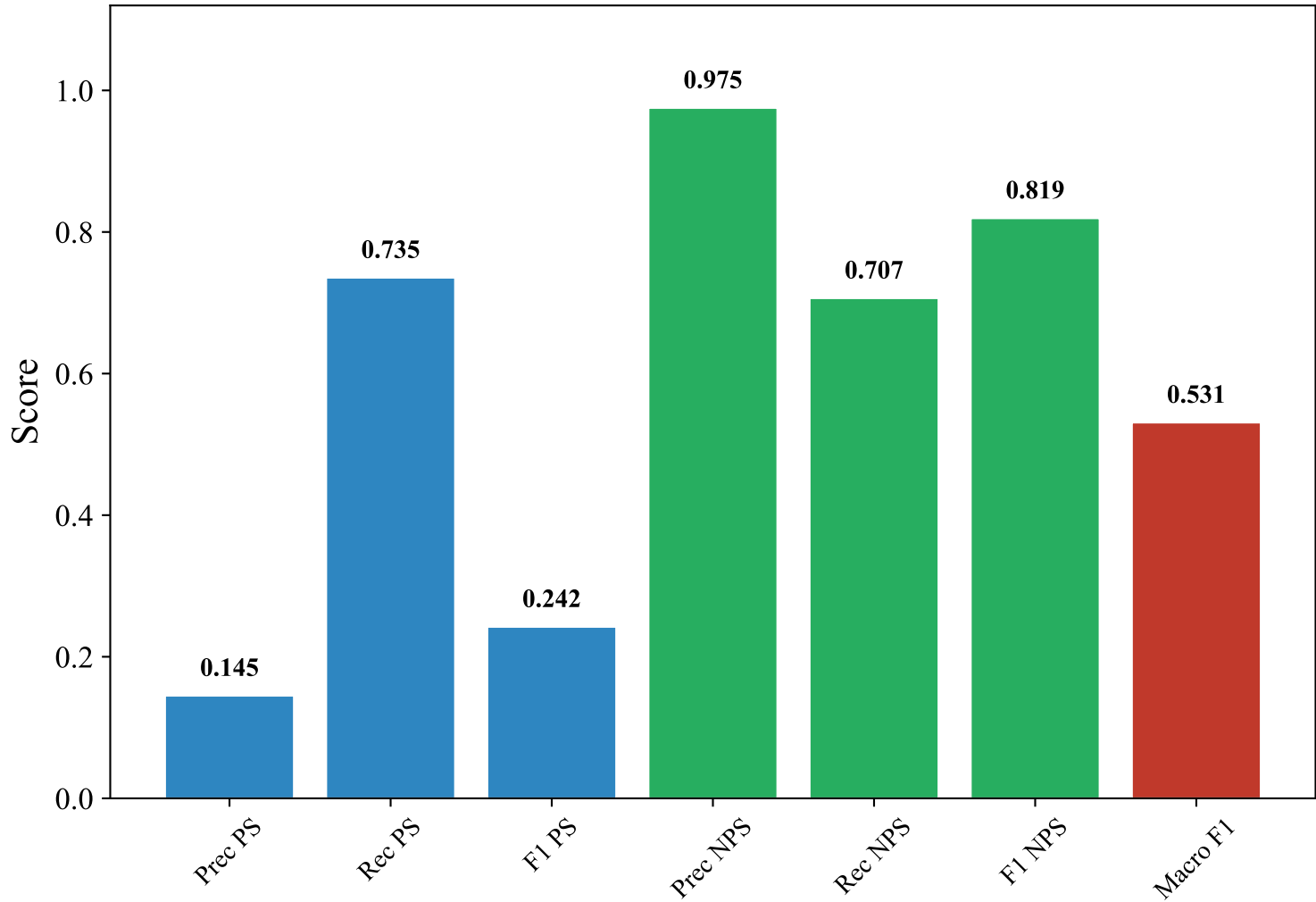
Classification Metrics — SWEDISH_MANUAL (snowflake-arctic-embed-l-v2.0, Random_Forest)
