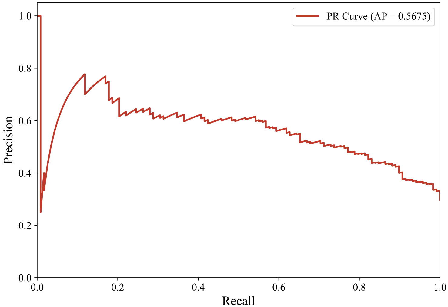
Precision-Recall Curve — DUTCH_MANUAL (paraphrase-multilingual-MiniLM-L12-v2, LightGBM_Optimized)
