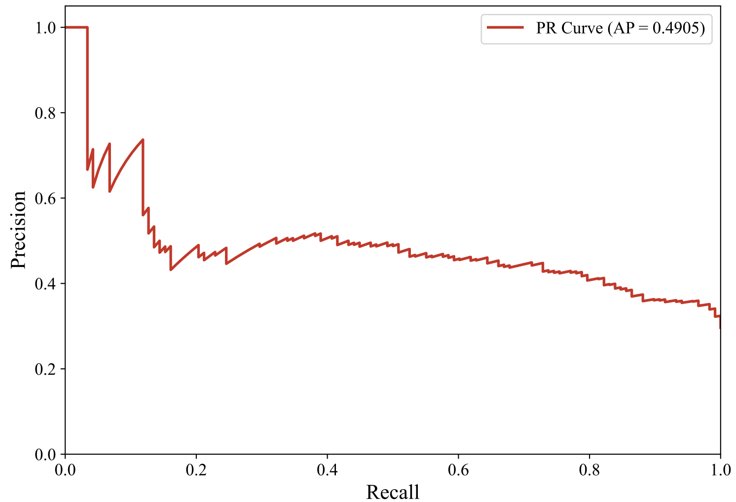
Precision-Recall Curve — DUTCH_MANUAL (paraphrase-multilingual-MiniLM-L12-v2, Random_Forest_Optimized)
