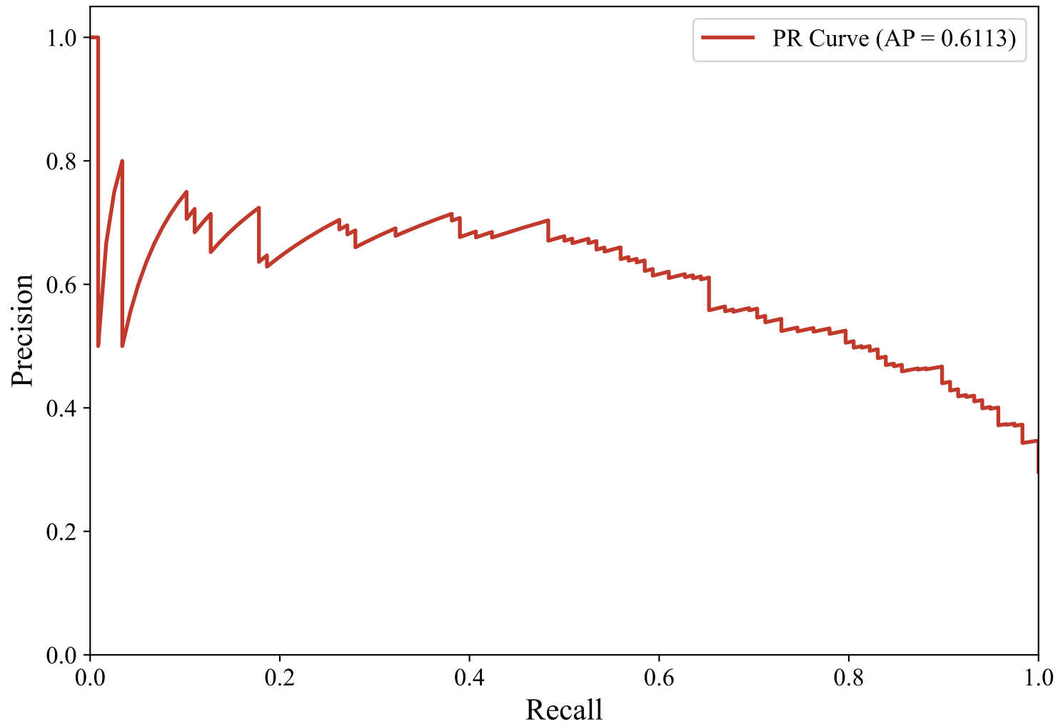
Precision-Recall Curve — DUTCH_MANUAL (paraphrase-multilingual-mpnet-base-v2, XGBoost_Optimized)
