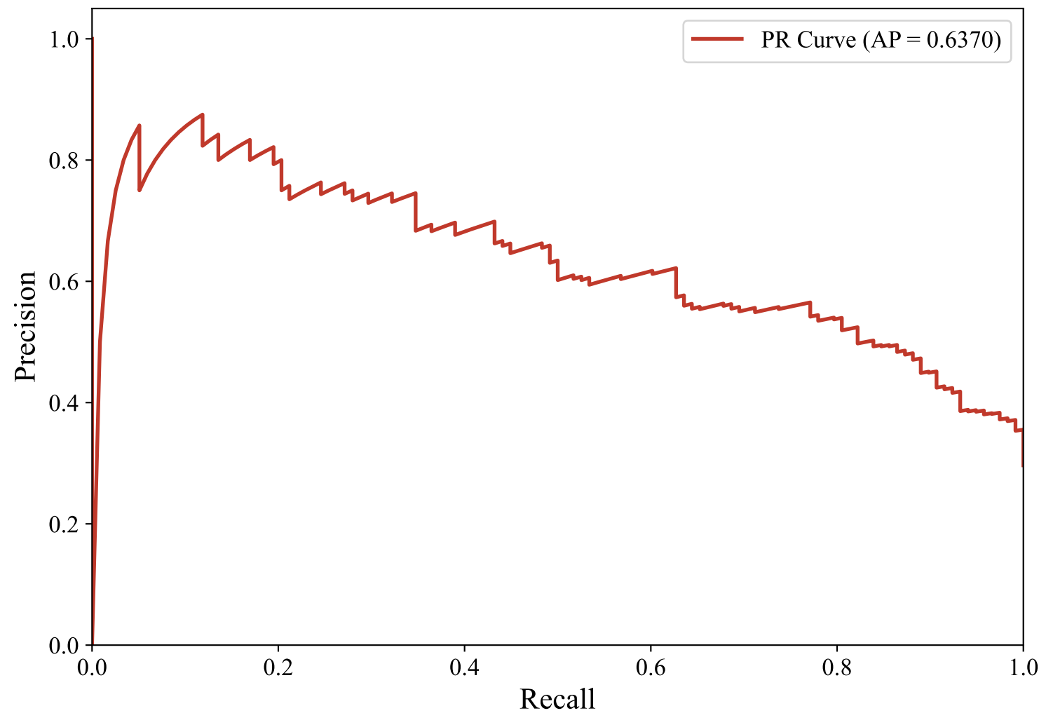
Precision-Recall Curve — DUTCH_MANUAL (snowflake-arctic-embed-l-v2.0, LightGBM_Optimized)
