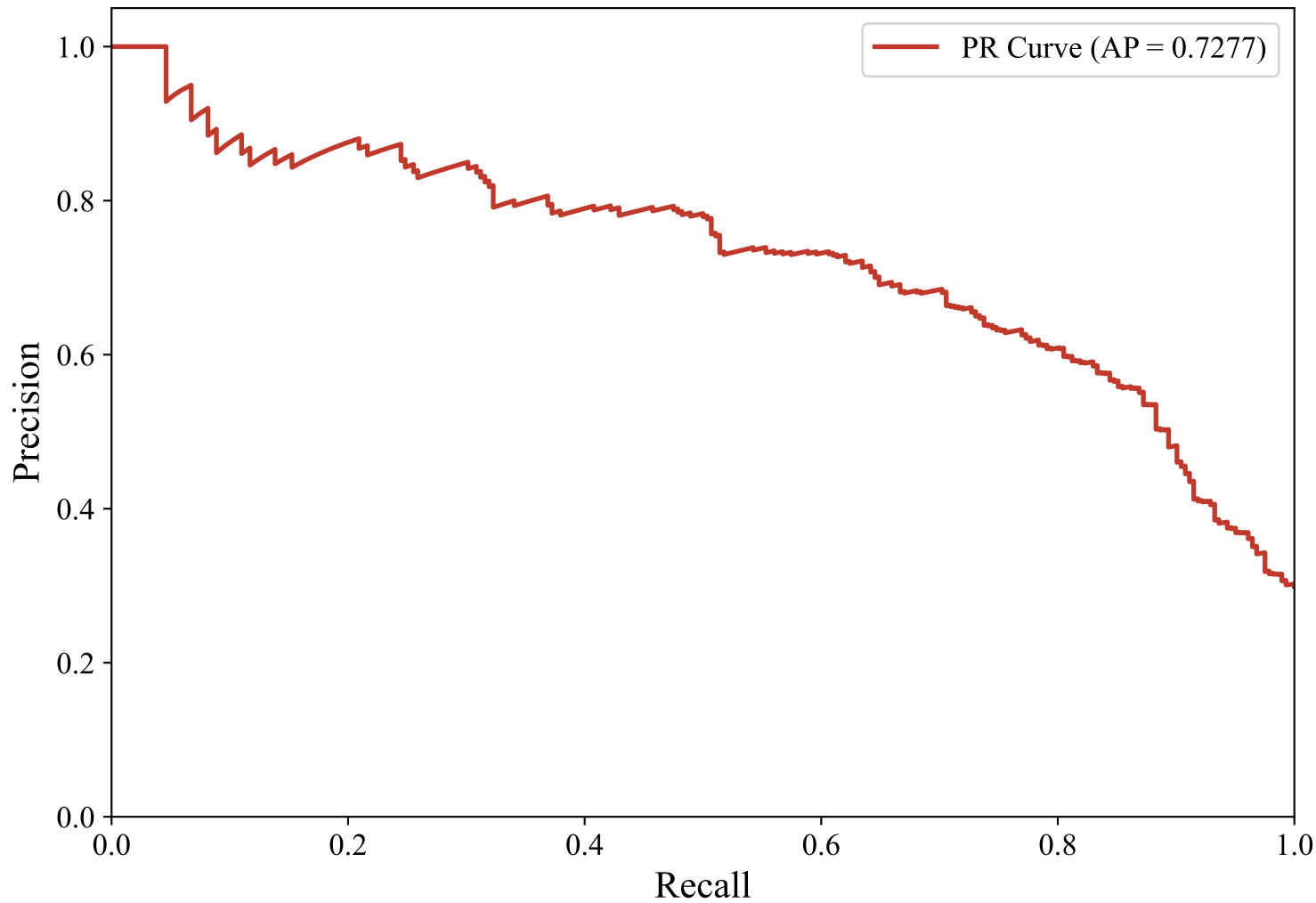
Precision-Recall Curve — ENGLISH_MANUAL (paraphrase-multilingual-MiniLM-L12-v2, LightGBM_Optimized)
