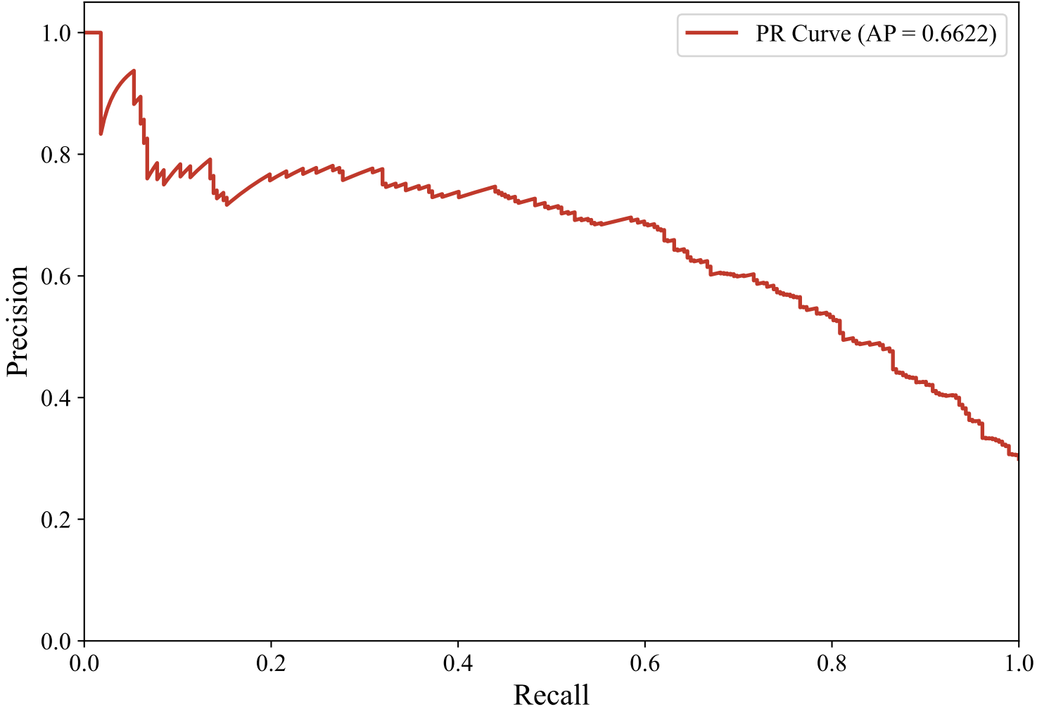
Precision-Recall Curve — ENGLISH_MANUAL (paraphrase-multilingual-MiniLM-L12-v2, Random_Forest)
