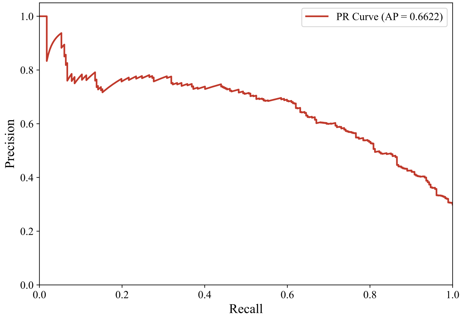
Precision-Recall Curve — ENGLISH_MANUAL (paraphrase-multilingual-MiniLM-L12-v2, Random_Forest_Optimized)
