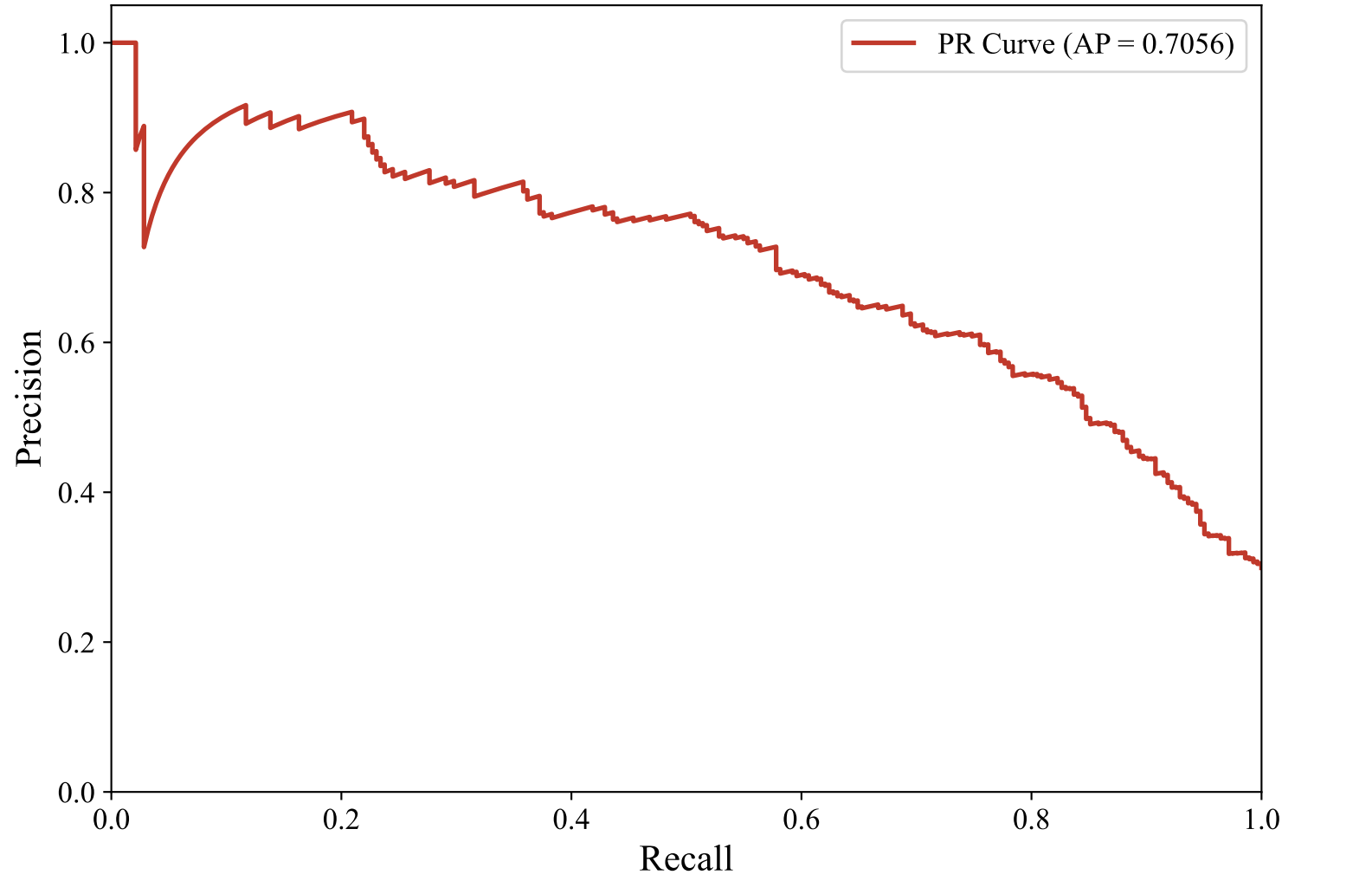
Precision-Recall Curve — ENGLISH_MANUAL (snowflake-arctic-embed-l-v2.0, Random_Forest_Optimized)
