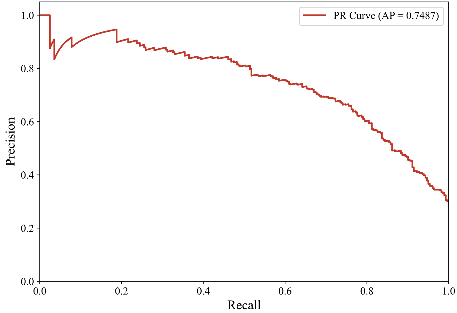
Precision-Recall Curve — ENGLISH_MANUAL (upskyy/bge-m3-korean, XGBoost_Optimized)
