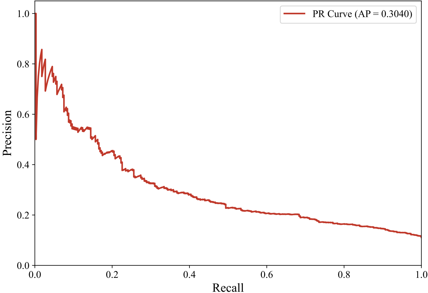
Precision-Recall Curve — GERMAN_MANUAL (paraphrase-multilingual-MiniLM-L12-v2, Random_Forest)
