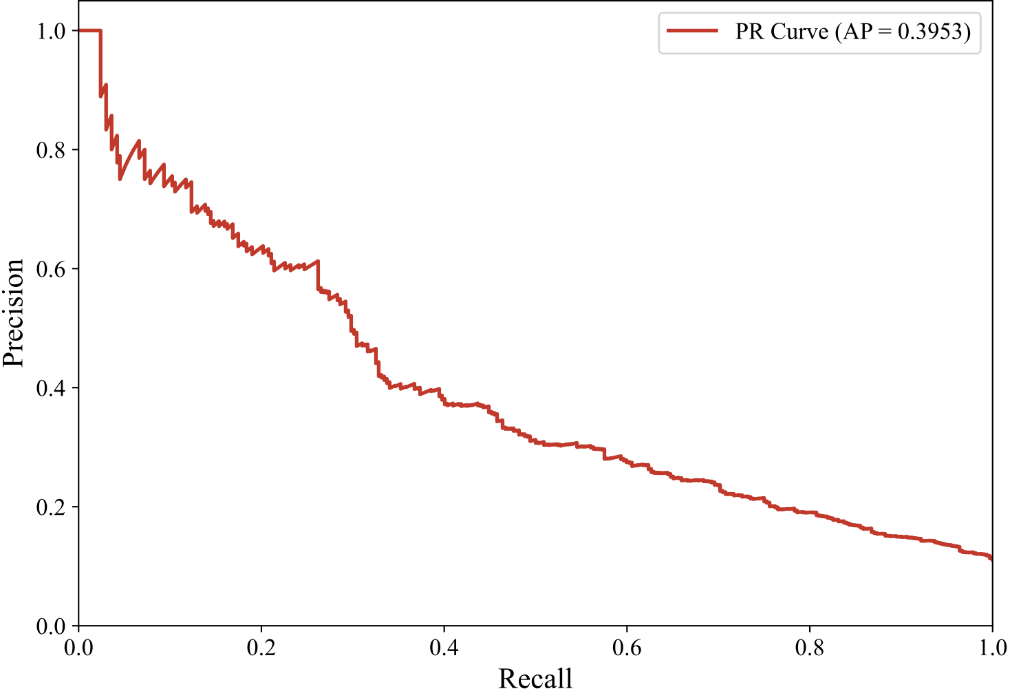
Precision-Recall Curve — GERMAN_MANUAL (paraphrase-multilingual-MiniLM-L12-v2, XGBoost_Optimized)
