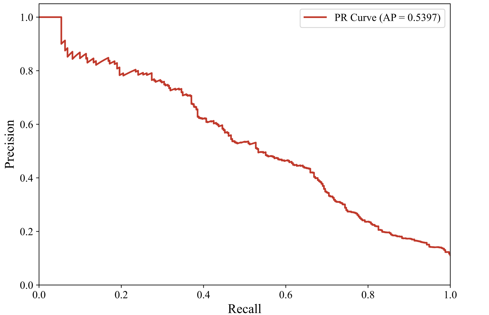
Precision-Recall Curve — GERMAN_MANUAL (snowflake-arctic-embed-l-v2.0, LightGBM_Optimized)
