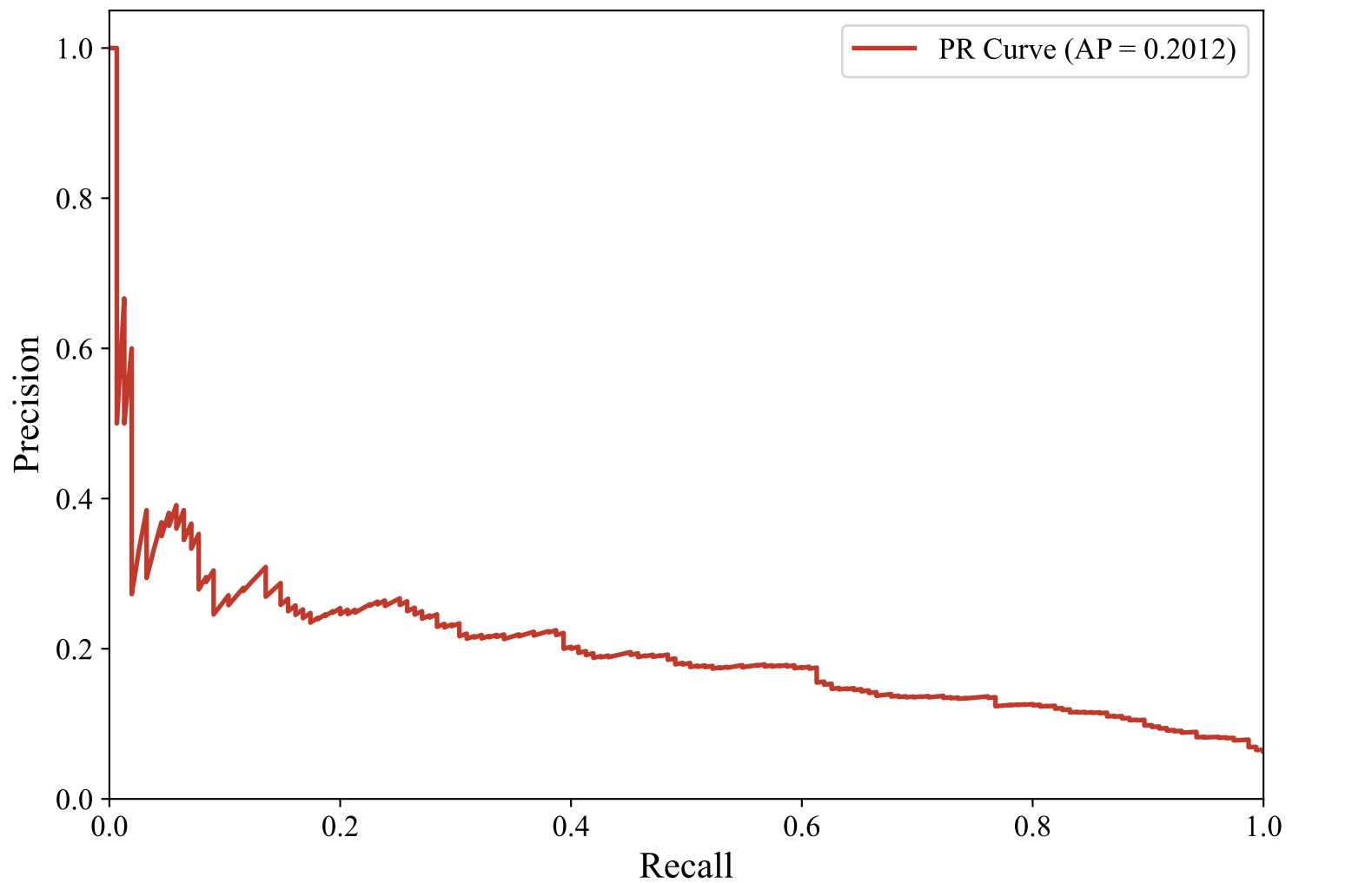
Precision-Recall Curve — SWEDISH_MANUAL (paraphrase-multilingual-MiniLM-L12-v2, LightGBM)
