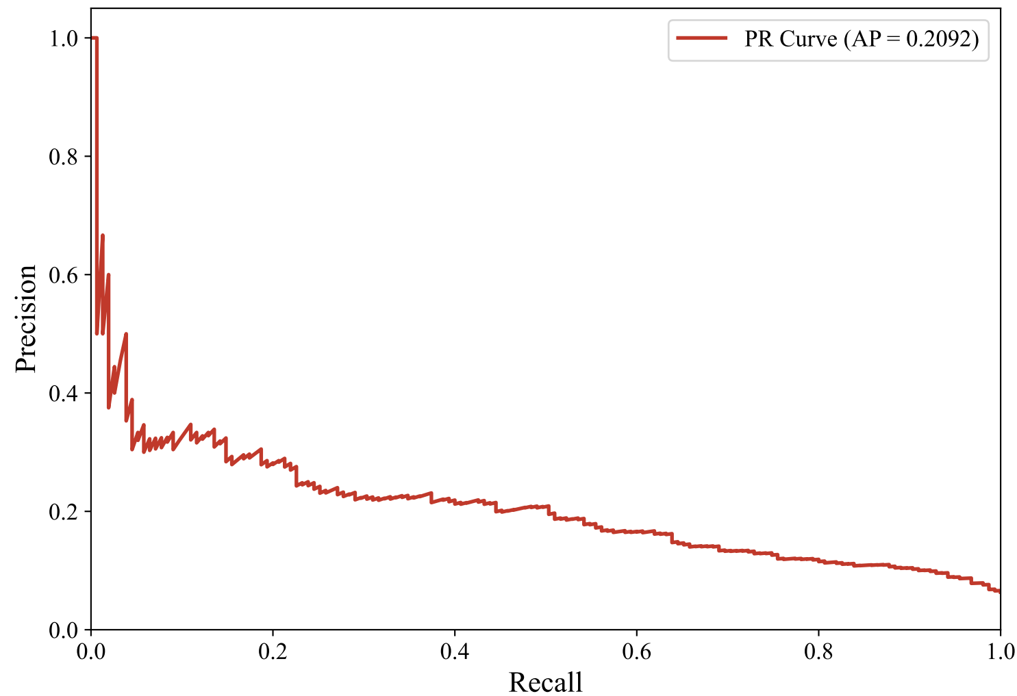
Precision-Recall Curve — SWEDISH_MANUAL (paraphrase-multilingual-MiniLM-L12-v2, XGBoost)
