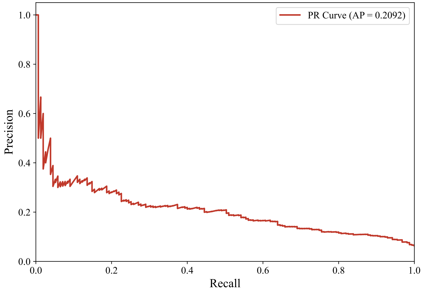
Precision-Recall Curve — SWEDISH_MANUAL (paraphrase-multilingual-MiniLM-L12-v2, XGBoost_Optimized)
