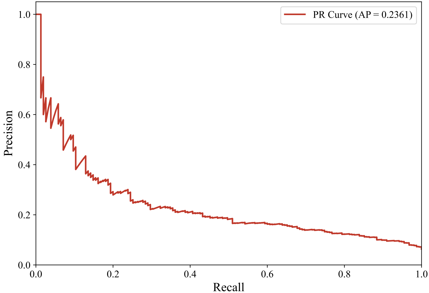
Precision-Recall Curve — SWEDISH_MANUAL (paraphrase-multilingual-mpnet-base-v2, LightGBM)
