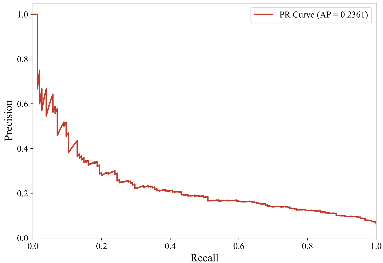
Precision-Recall Curve — SWEDISH_MANUAL (paraphrase-multilingual-mpnet-base-v2, LightGBM_Optimized)
