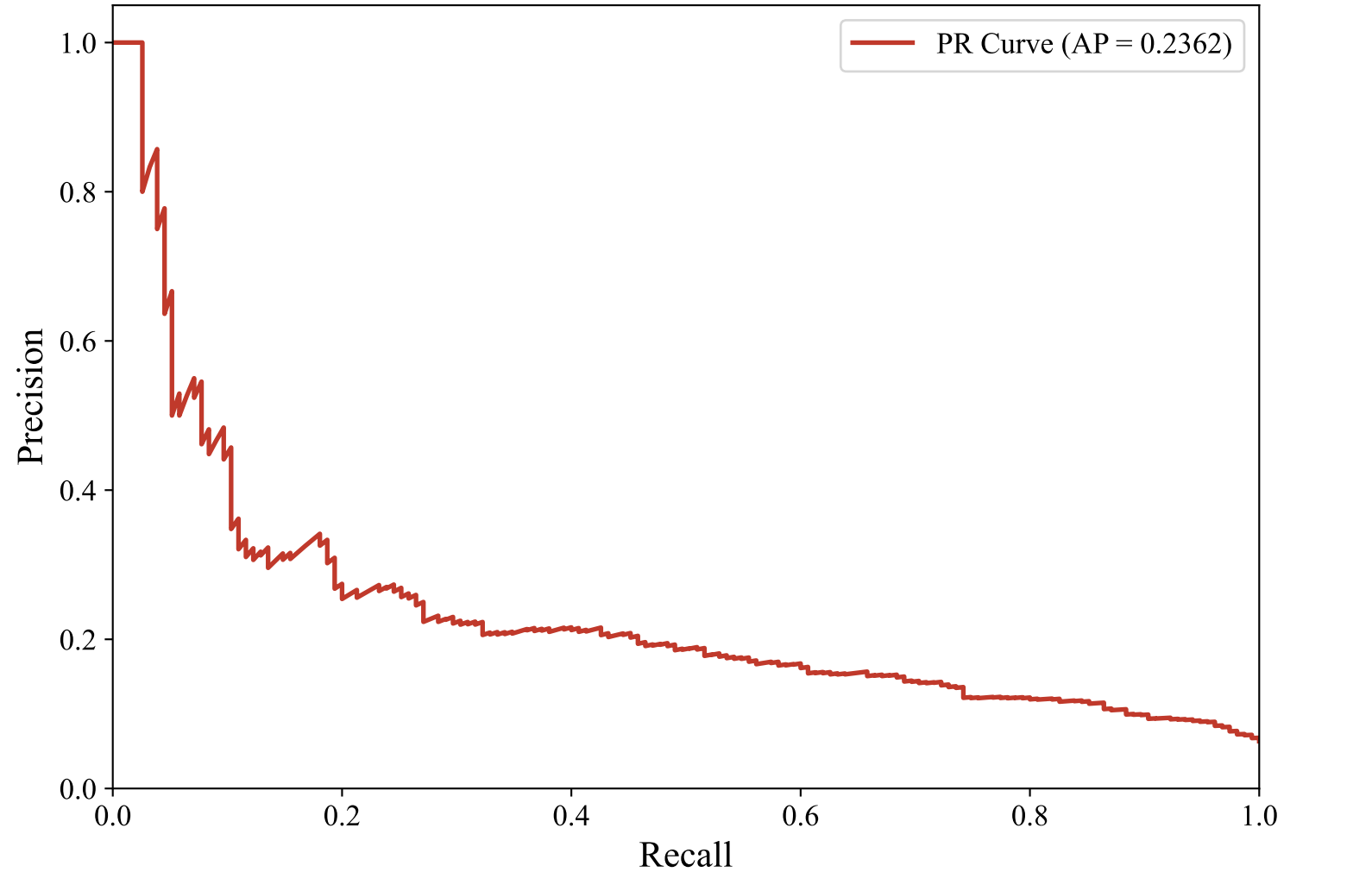
Precision-Recall Curve — SWEDISH_MANUAL (paraphrase-multilingual-mpnet-base-v2, XGBoost)
