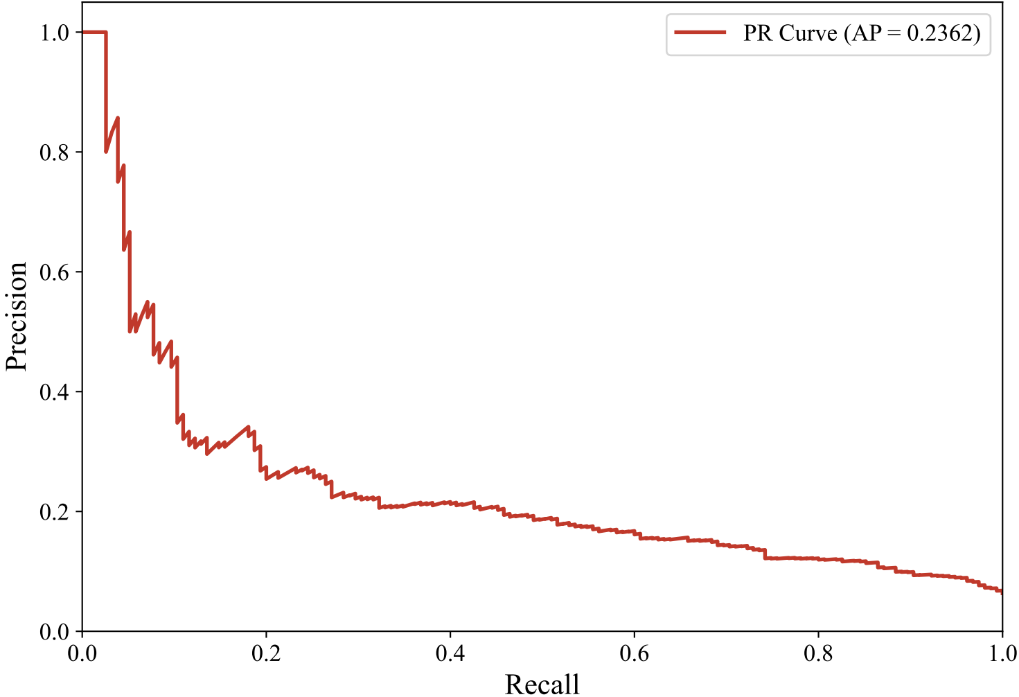
Precision-Recall Curve — SWEDISH_MANUAL (paraphrase-multilingual-mpnet-base-v2, XGBoost_Optimized)
