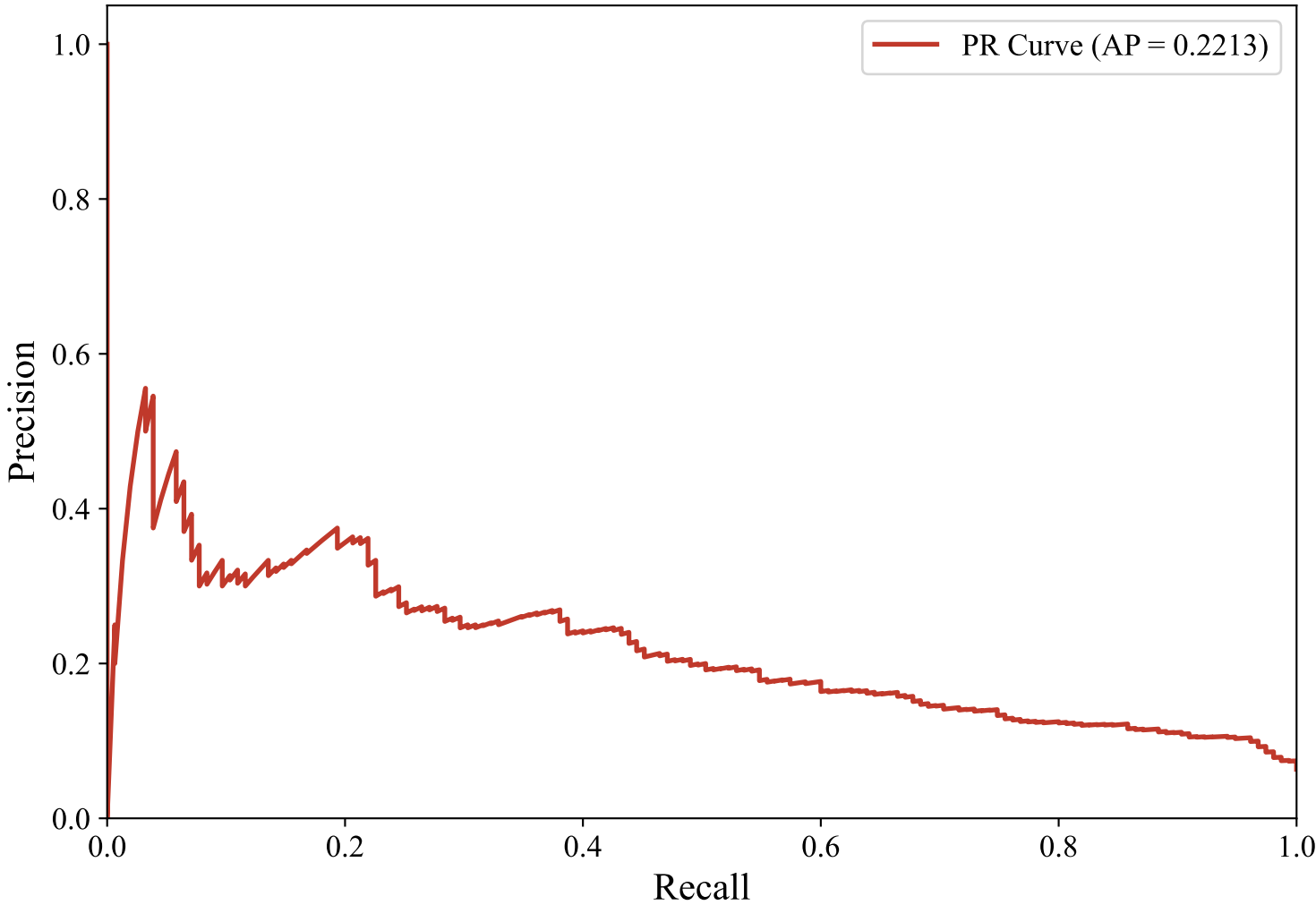
Precision-Recall Curve — SWEDISH_MANUAL (snowflake-arctic-embed-l-v2.0, LightGBM)
