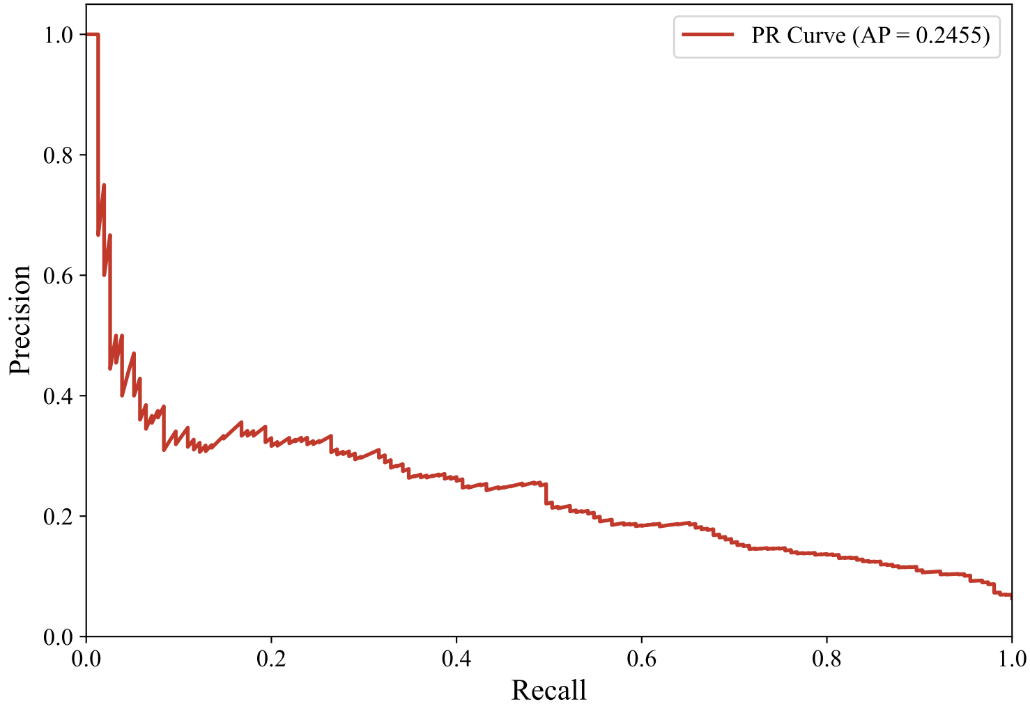
Precision-Recall Curve — SWEDISH_MANUAL (snowflake-arctic-embed-l-v2.0, XGBoost_Optimized)
