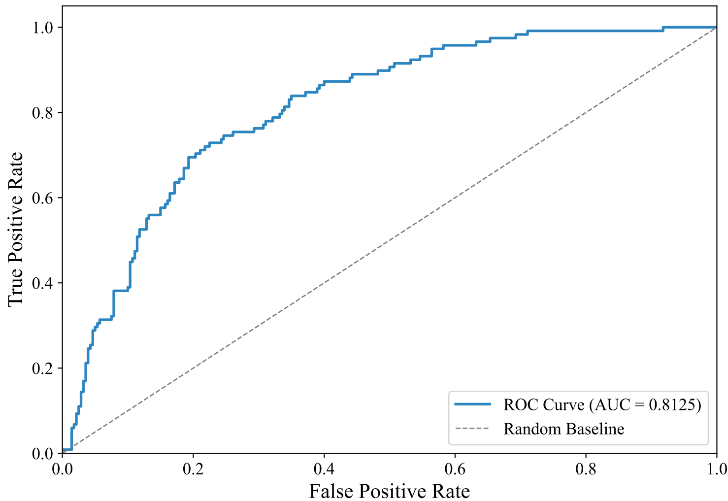
ROC Curve — DUTCH_MANUAL (paraphrase-multilingual-mpnet-base-v2, LightGBM)
