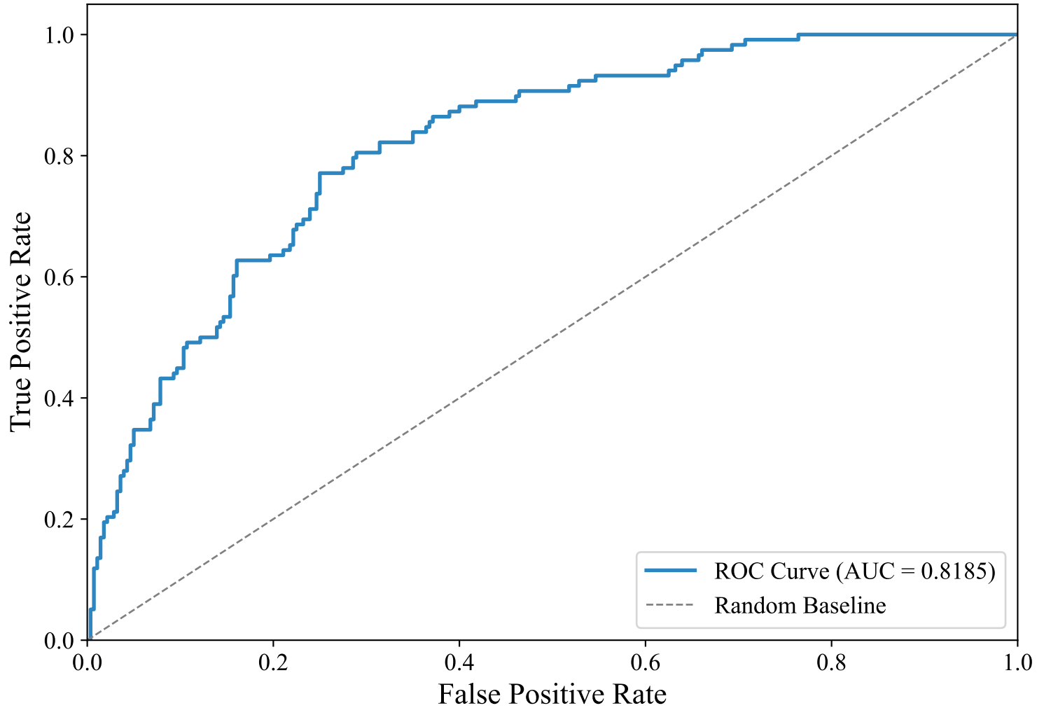
ROC Curve — DUTCH_MANUAL (snowflake-arctic-embed-l-v2.0, LightGBM_Optimized)
