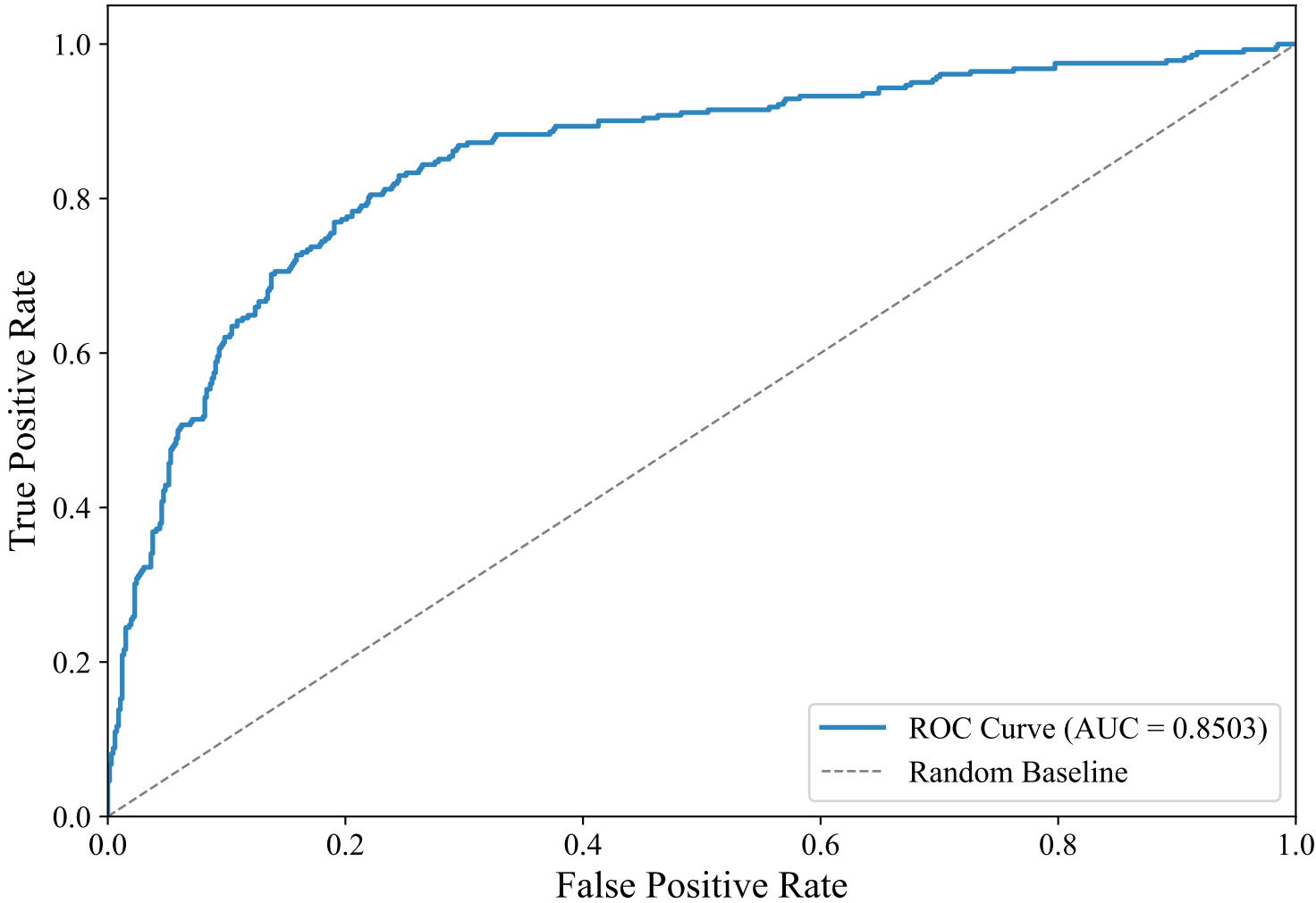
ROC Curve — ENGLISH_MANUAL (paraphrase-multilingual-MiniLM-L12-v2, LightGBM)
