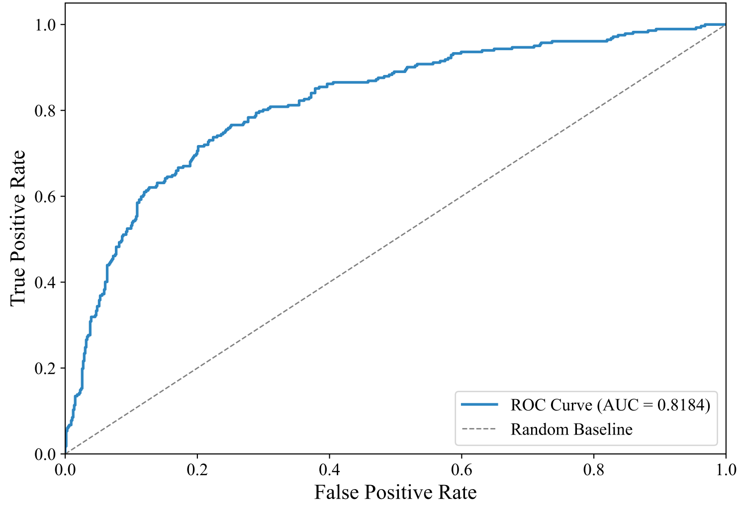
ROC Curve — ENGLISH_MANUAL (paraphrase-multilingual-MiniLM-L12-v2, Random_Forest)
