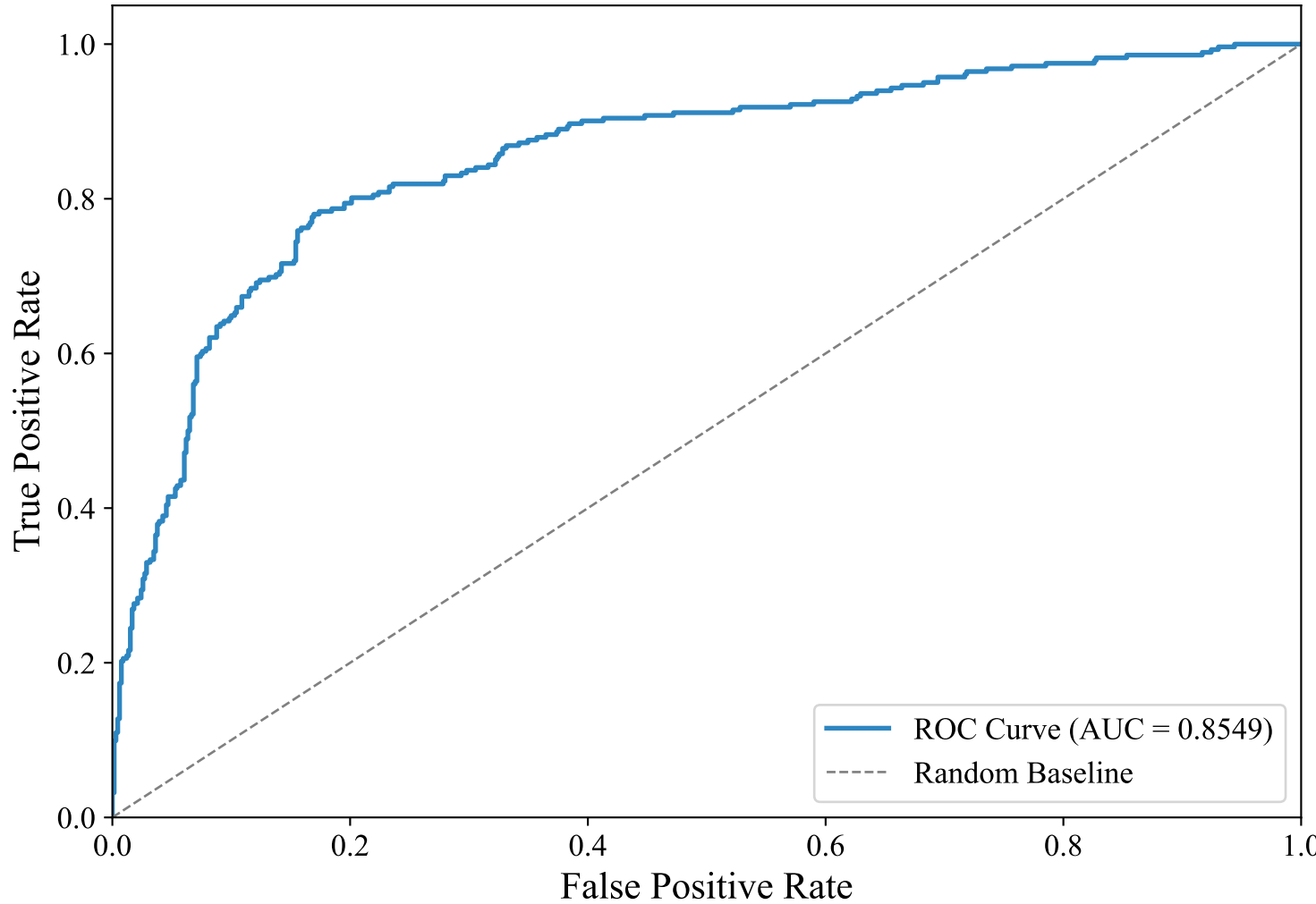
ROC Curve — ENGLISH_MANUAL (paraphrase-multilingual-MiniLM-L12-v2, XGBoost_Optimized)
