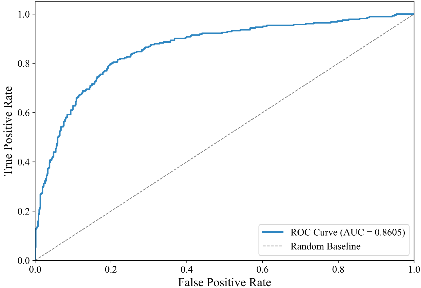
ROC Curve — ENGLISH_MANUAL (snowflake-arctic-embed-l-v2.0, LightGBM_Optimized)
