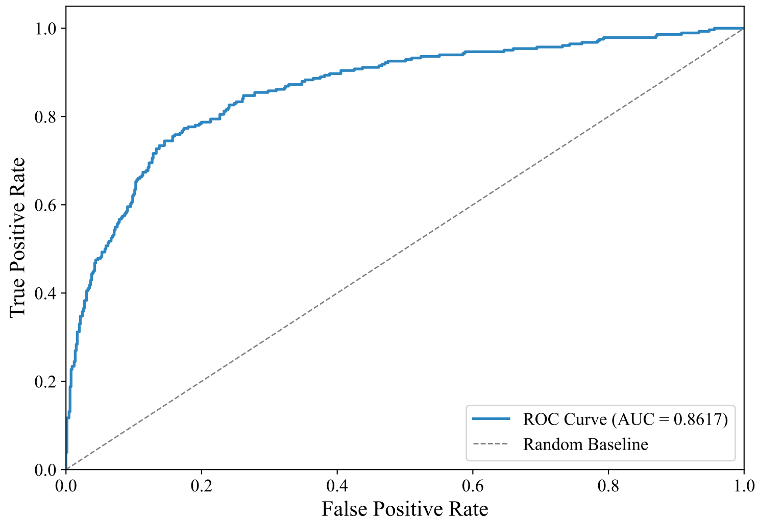
ROC Curve — ENGLISH_MANUAL (snowflake-arctic-embed-l-v2.0, XGBoost)
