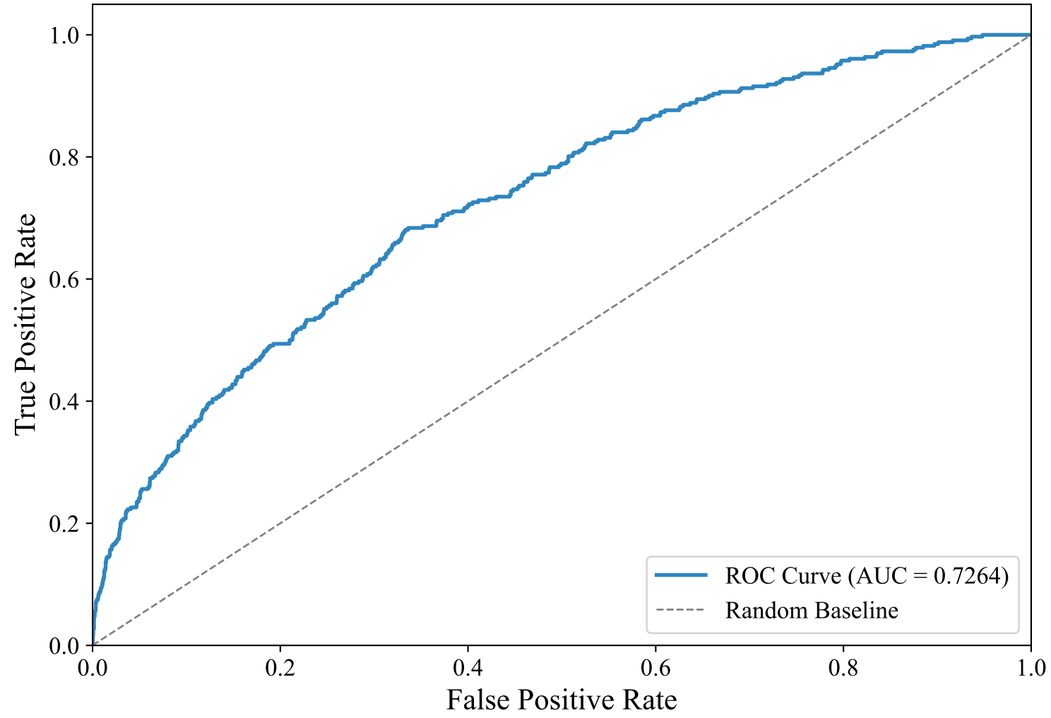
ROC Curve — GERMAN_MANUAL (paraphrase-multilingual-MiniLM-L12-v2, Random_Forest)
