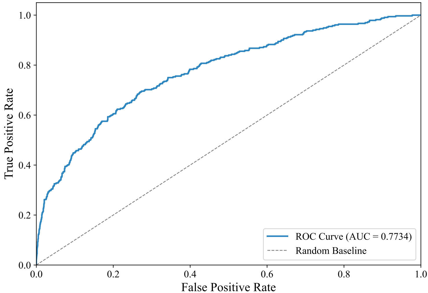
ROC Curve — GERMAN_MANUAL (paraphrase-multilingual-MiniLM-L12-v2, XGBoost_Optimized)
