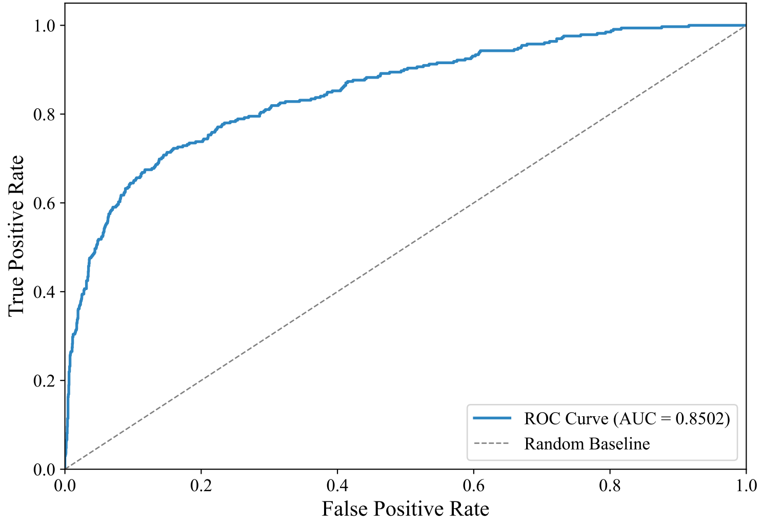
ROC Curve — GERMAN_MANUAL (snowflake-arctic-embed-l-v2.0, Voting_Ensemble)
