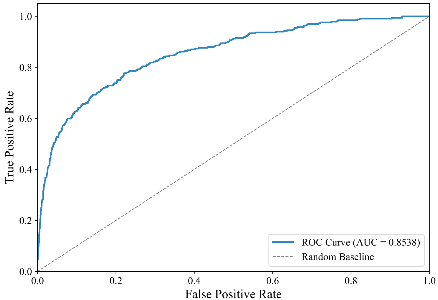
ROC Curve — GERMAN_MANUAL (snowflake-arctic-embed-l-v2.0, XGBoost_Optimized)
